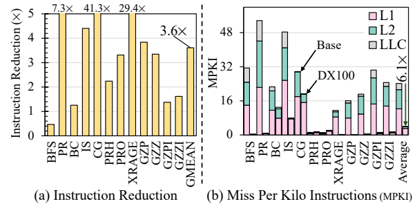
Figure 11: DX100 (a) instruction and (b) MPKI reduction.
